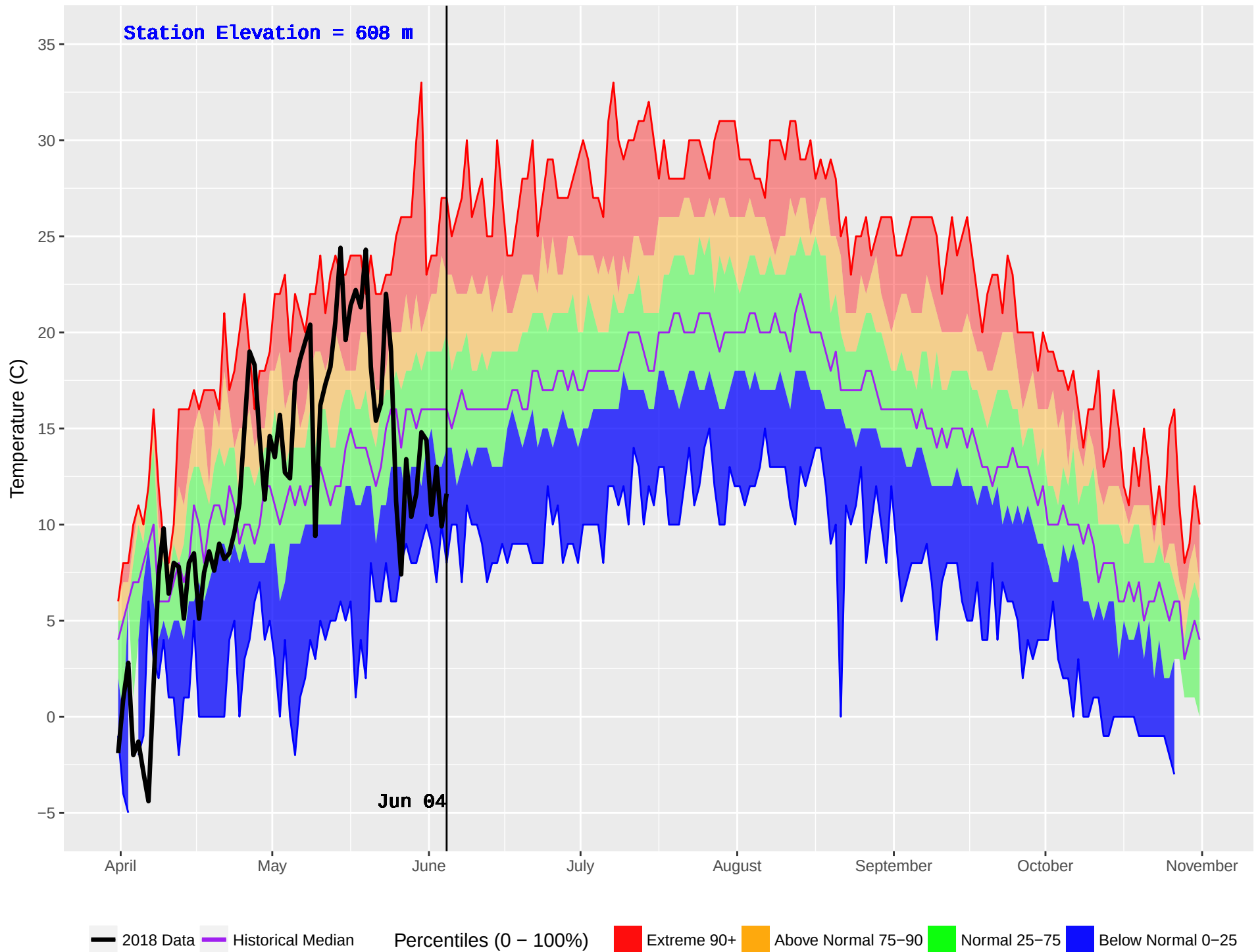
HOUSTON(DUNGATE) (162) : Historical (1974–2016) and Current (2018) Noon Temperature
