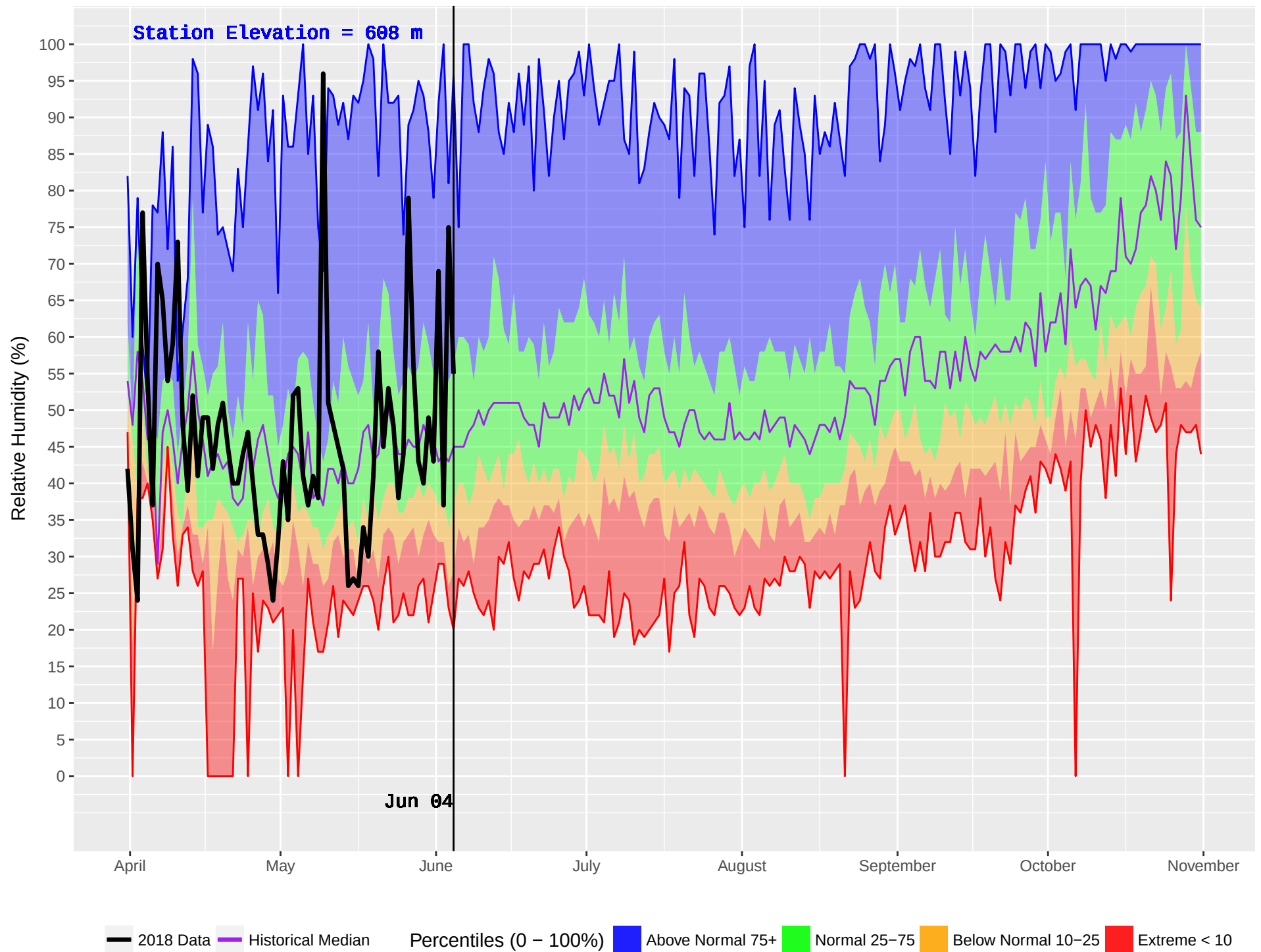
HOUSTON(DUNGATE) (162) : Historical (1974–2016) and Current (2018) Noon Relative Humidity
