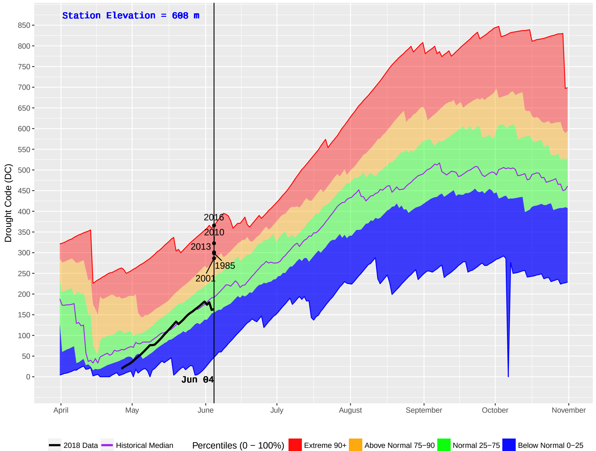
HOUSTON(DUNGATE) (162) : Historical (1974–2016) and Current (2018) Noon Drought Code (DC)
